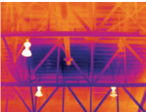
Interior IR survey conducted during daylight hours reveals central area saturated with moisture and in need of repair.
