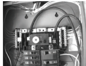
Hot lug in a service panel.
